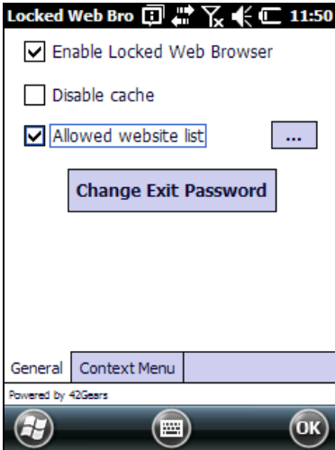
General Tab
