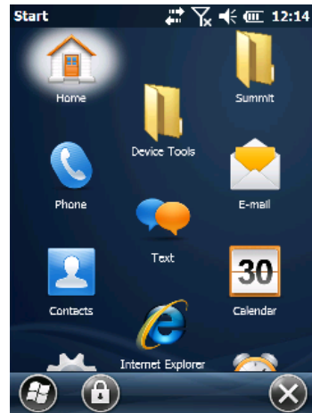
Start Menu
