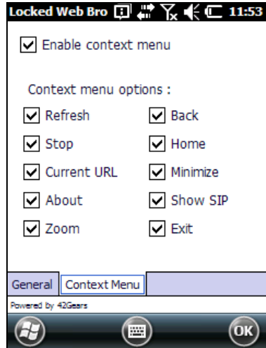
Context Menu
