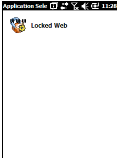
Application Selector
