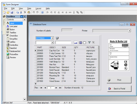
Form Designer
